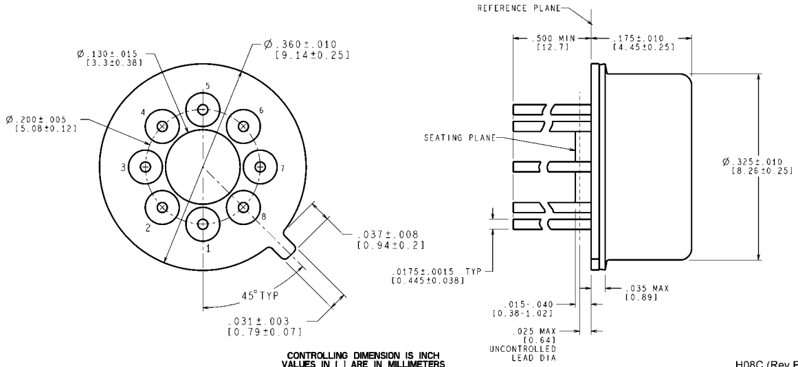
TO-99 Metal Can Package Order Number LME49720HA NS Package Number H08C
